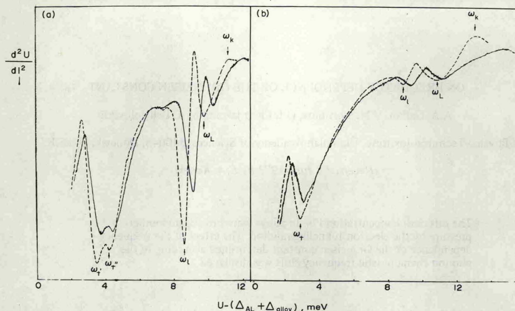
Fig. 1. (d^2U/dl^2) - U characteristics at P = 0 (the dashed line) and P = 9.3 kbar, T \sim 1.2^\circ \text{K} . (a) \text{Pb}_{88}\text{In}_{12} ; (b) \text{Pb}_{60}\text{In}_{40} .
